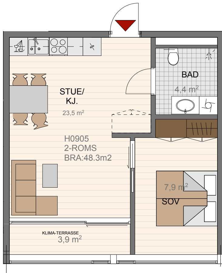
Leil Type 5A (2 roms)
